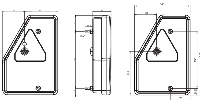
6 PIN BAYONET
