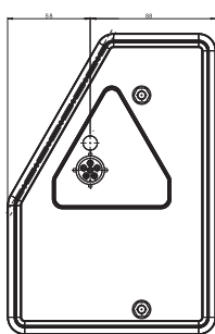
6 PIN BAYONET
